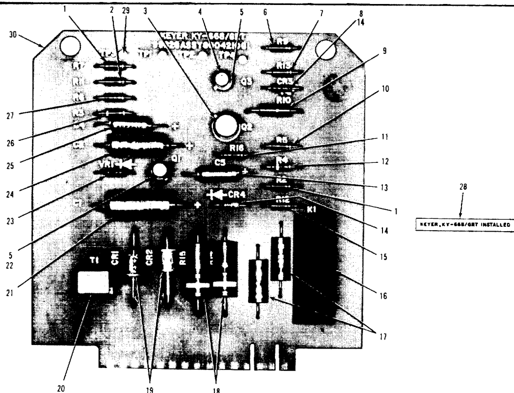
Figure 26. Keyer, KY-668/GRT (FOR NAVY ONLY)
