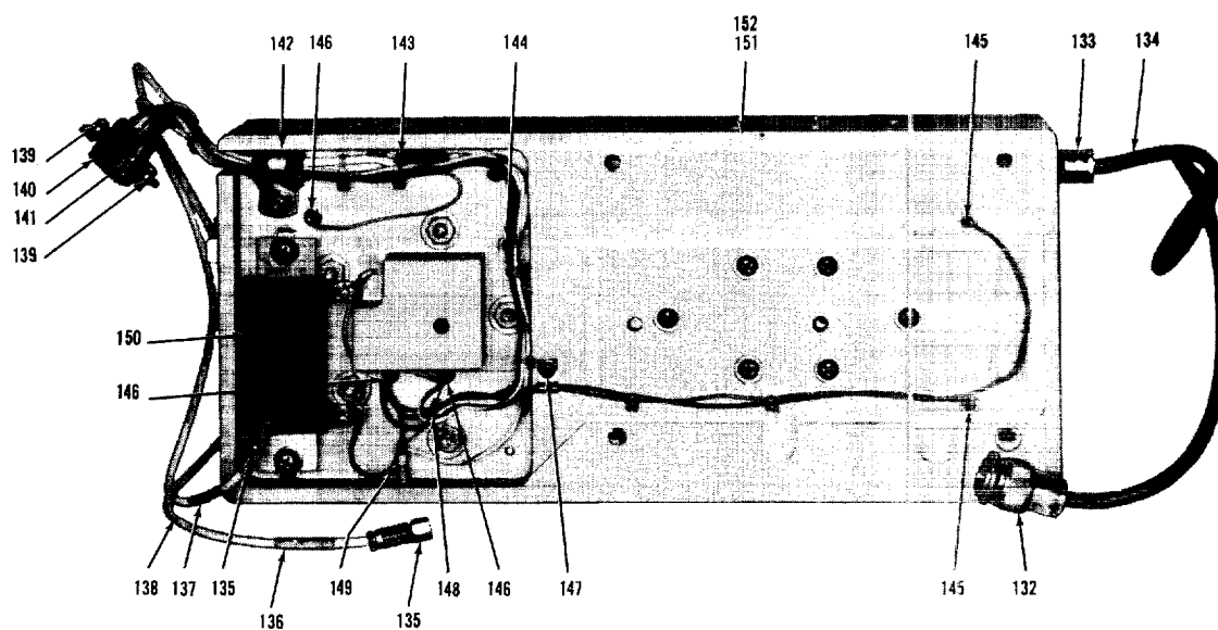
Figure 12. Amplifier, Driver/Power, RF, UHF (Sheet 2 of 2)
