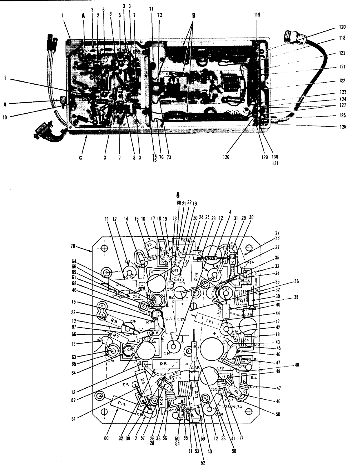
Figure 12. Amplifier, Driver/Power, RF, UHF (Sheet 1 of 2)
