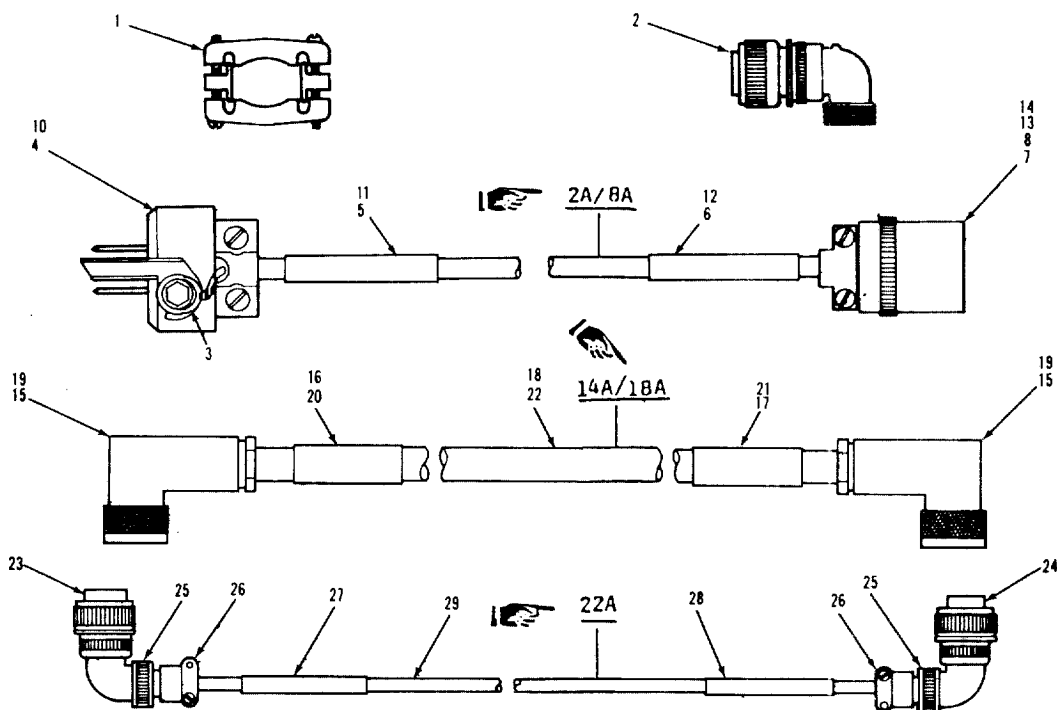
Figure 27. Interface Cable Kit
