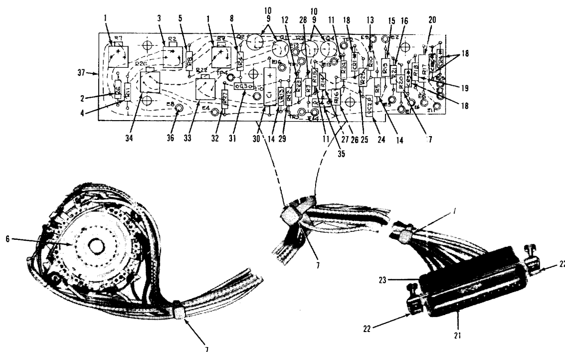
Figure 24. Buffer Amplifier/Multiplier, Electrical Instrument
