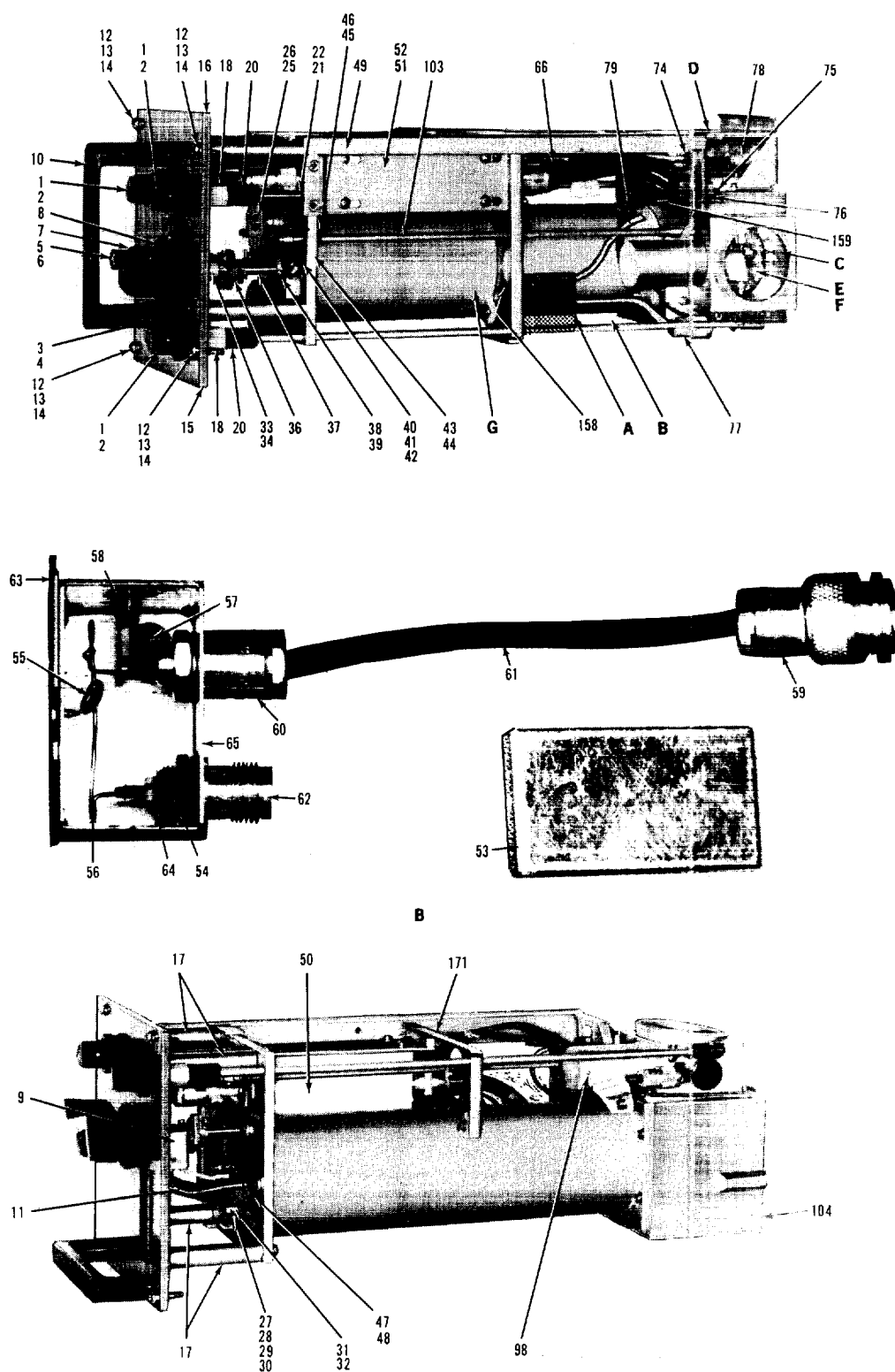
Figure 22. Cavity Assembly, Tuned (Sheet 1 of 3)
