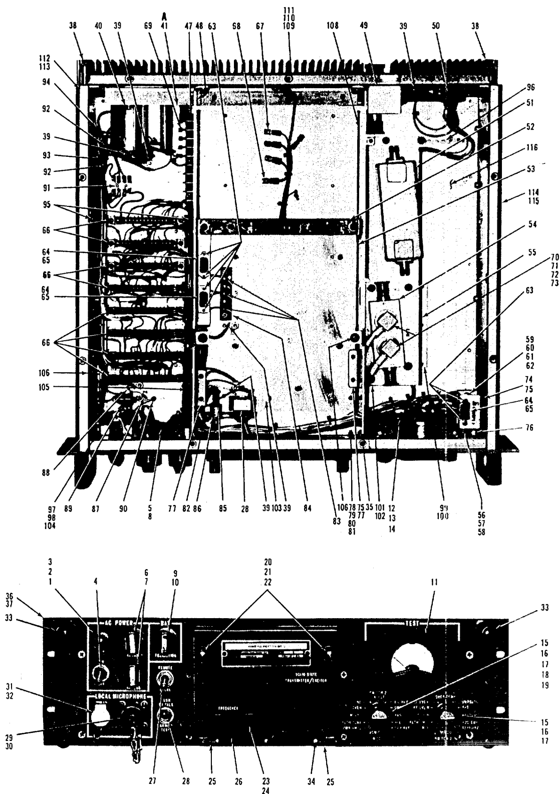
Figure 18. Frame Assembly, Transmitter, UHF and VHF (Sheet 1 of 2)
